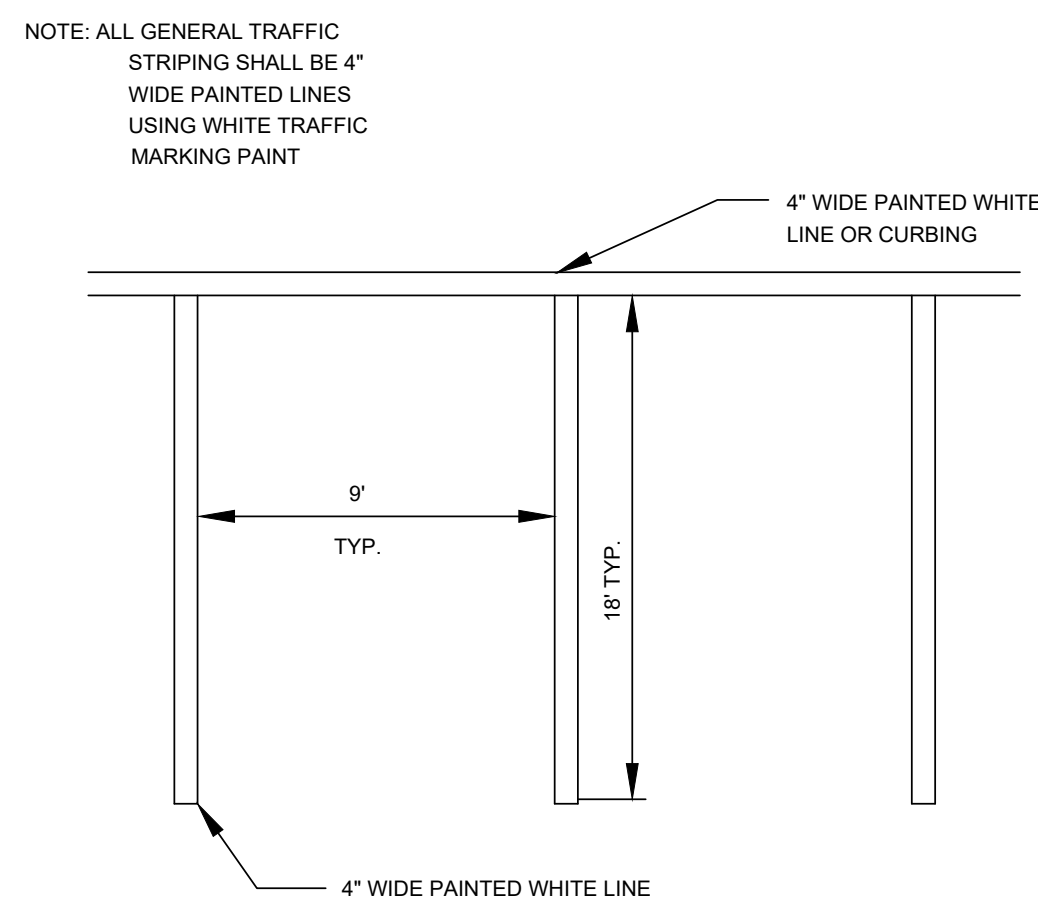
PARKING SPACE LAYOUT
