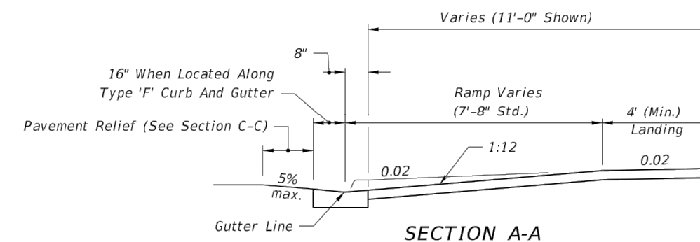
SECTION THROUGH RAMP AND LANDING (UNRESTRICTED CONDITIONS)
