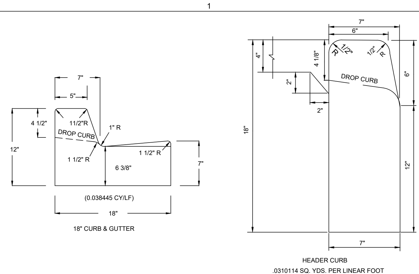
TYPICAL CURB DETAILS
