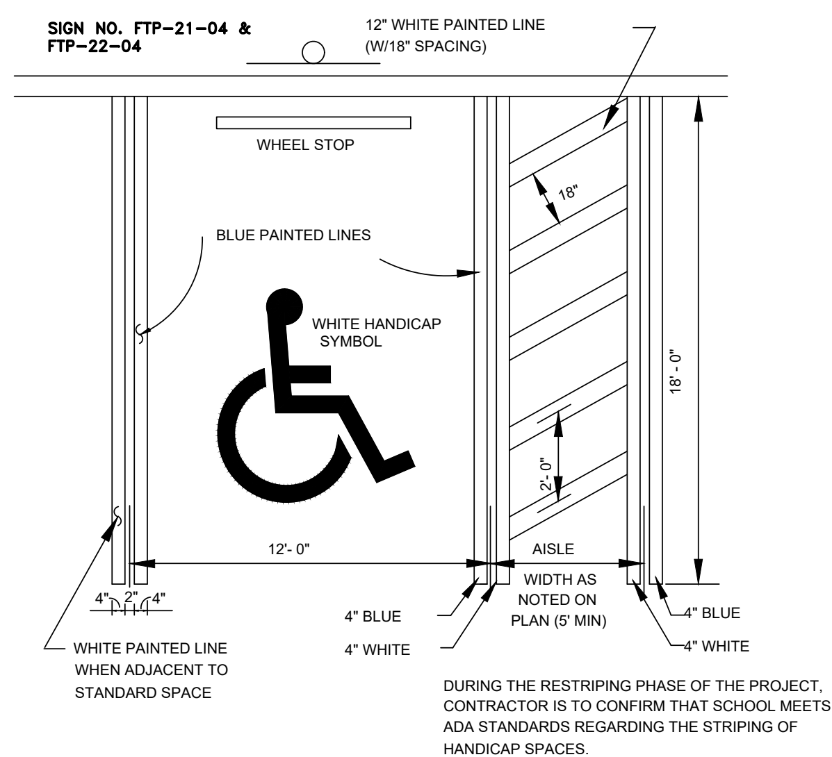
HANDICAP PARKING AND STRIPING
