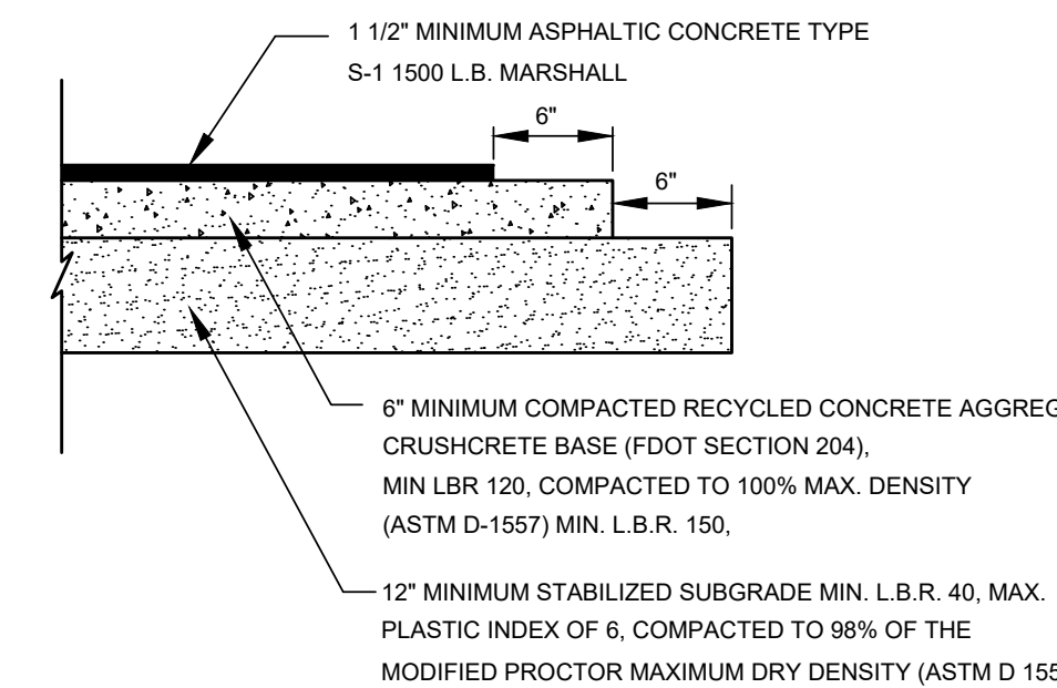
ASPHALT PAVEMENT SECTION W / CRUSHCRETE
