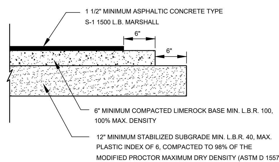
ASPHALT PAVEMENT SECTION-LIGHT DUTY
