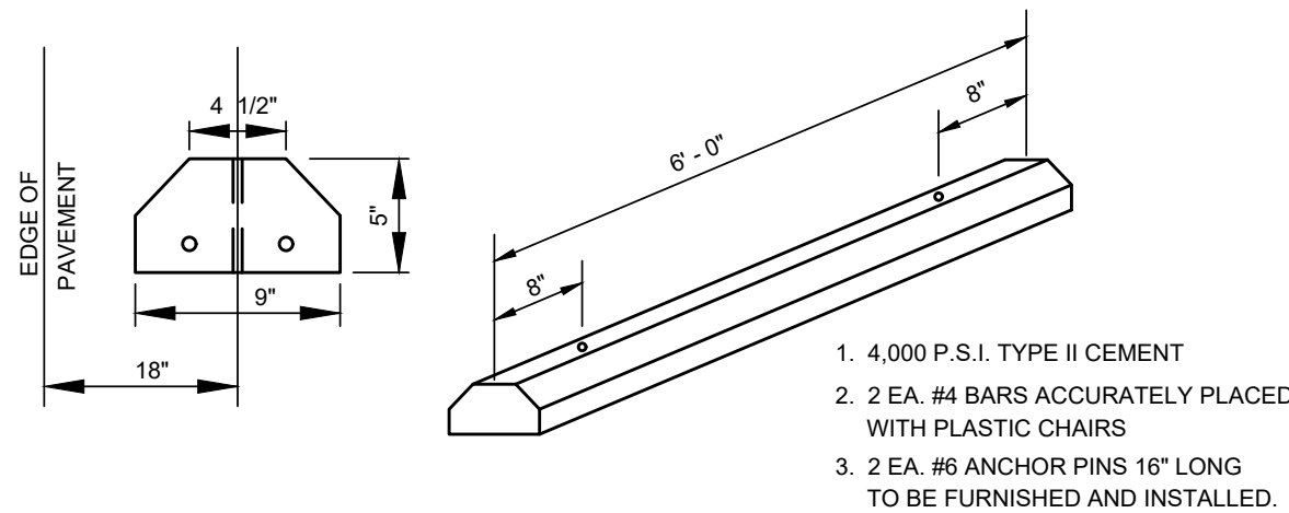
WHEEL STOP DETAIL
