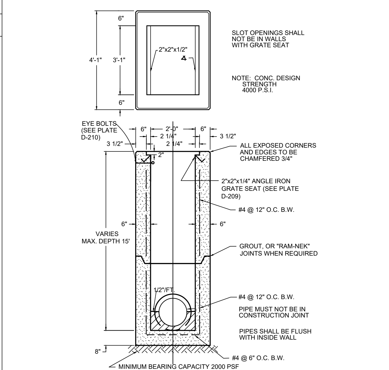
STANDARD CURB INLET
