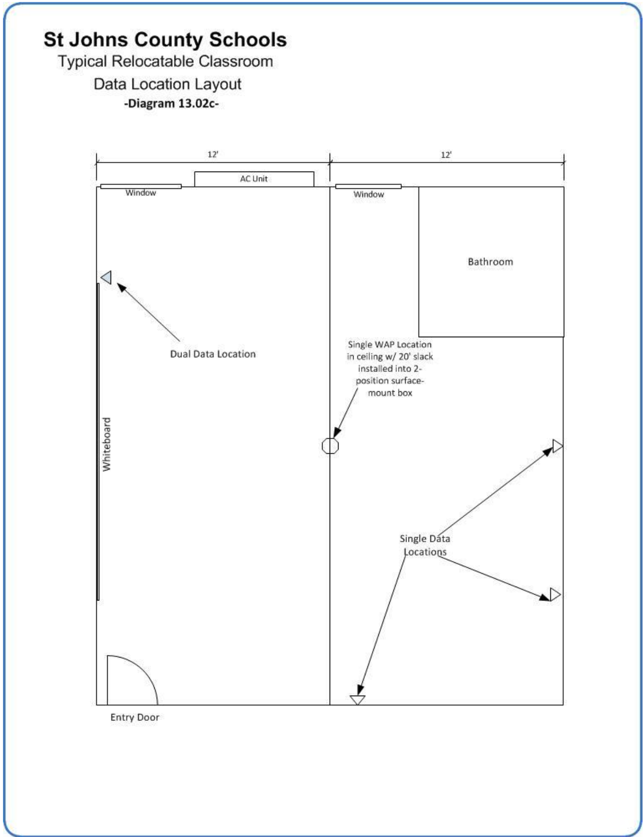
Diagram 13.02c – Typical Relocatable Work Area Outlet Layout
