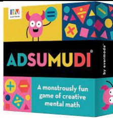
Adsumudi
