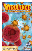
Virulence
