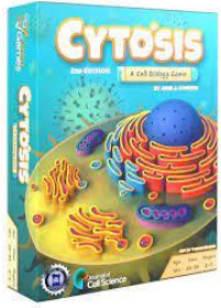
Cytosis
